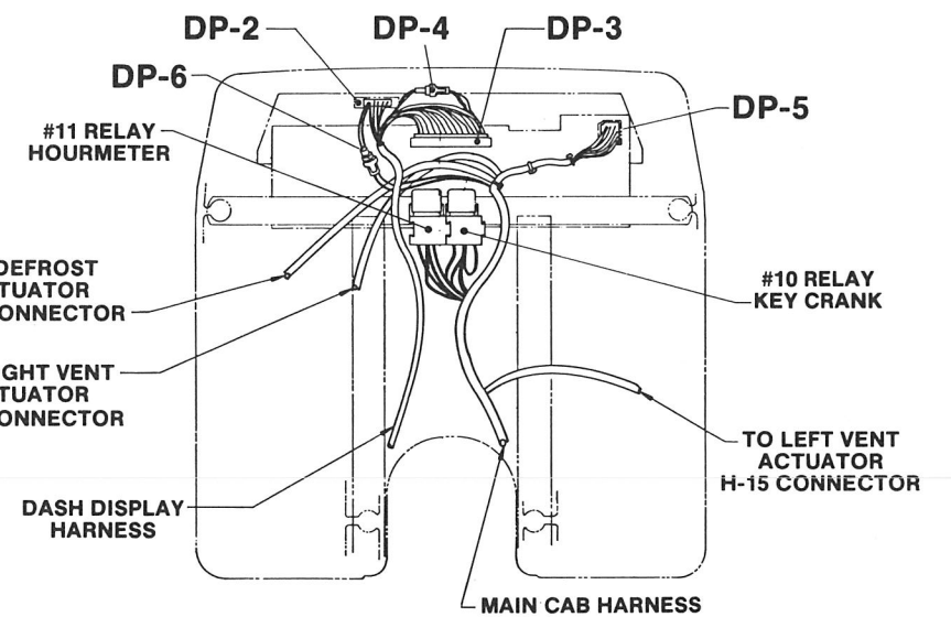
DASH ASSEMBLY - REAR VIEW
