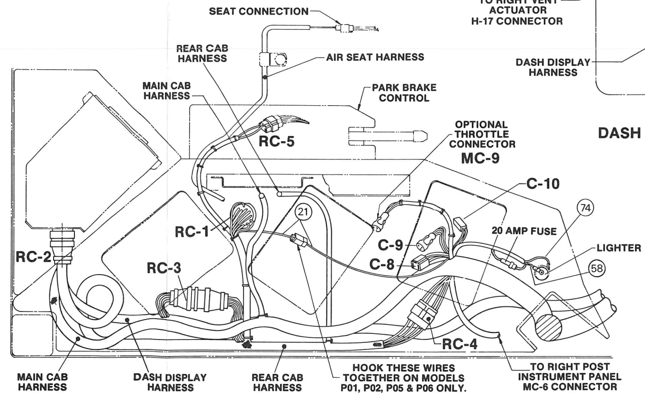
RIGHT SIDE CONTROL CONSOLE - TOP VIEW
