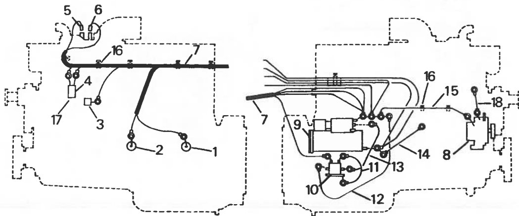
Bulkhead Connectors
