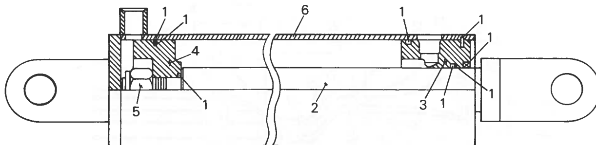
Pipe Ports
