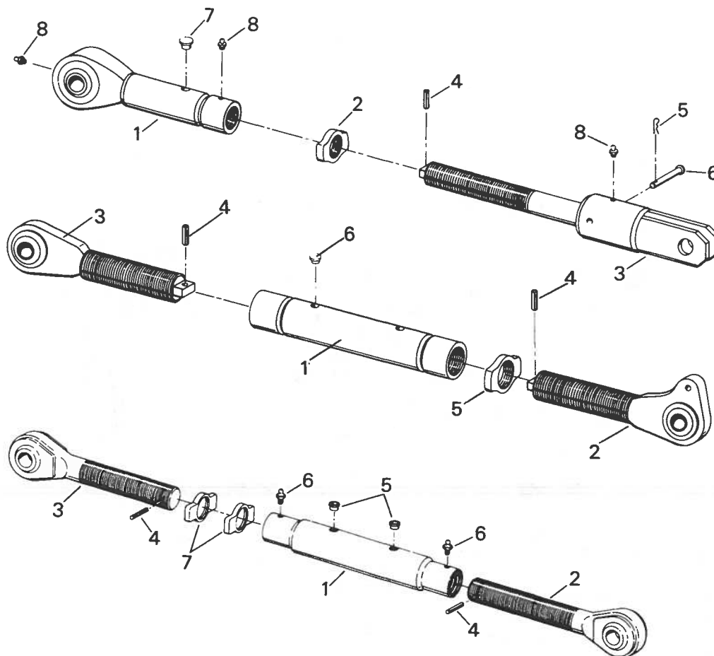
Adjusting Arm
