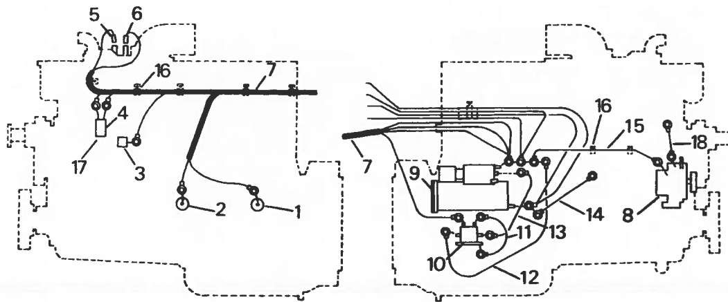
Bulkhead Connectors
