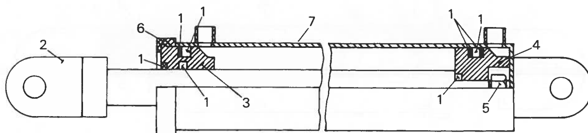
O-Ring Ports
