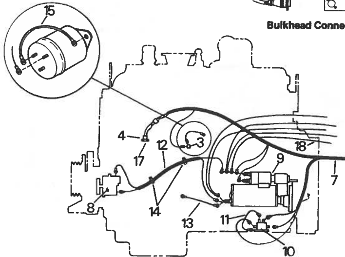
Packard Connectors
