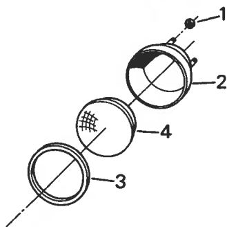
Headlamp Assembly
