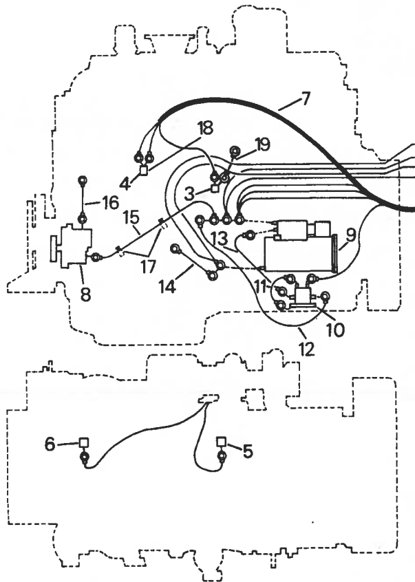
Packard Connectors
